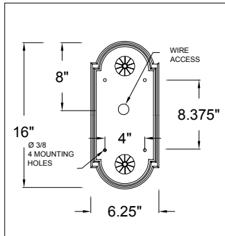
MOUNTING PLATE DETAIL
