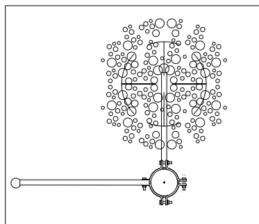
FLOWER BASKET BRACKET AND BANNER ARM ORIENTATION (TOP VIEW)
