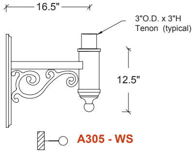
Weight: 8 lbs
